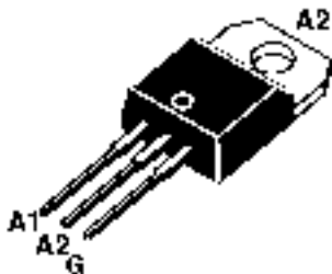
TO-220AB (BTB24)
